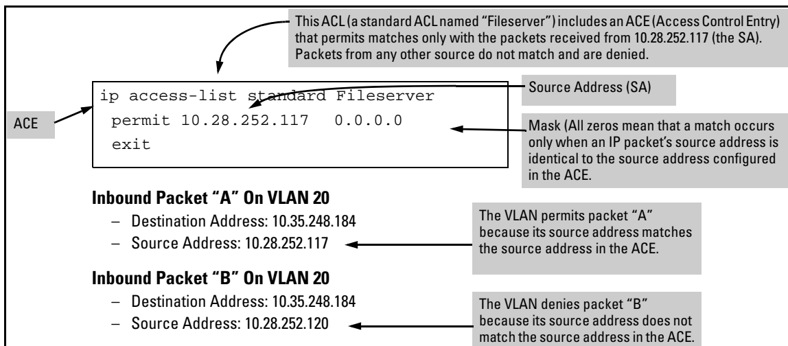
Figure 9-5. Example of an ACL with an Access Control Entry (ACE) that Allows Only One Source Address
